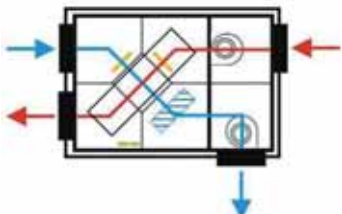
CADB/CADT-DC 05 / 08 / 18 / 30 / 45 / 56 EH DP BP MODELS
