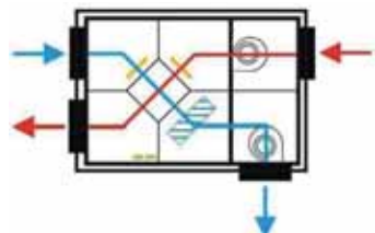
MODELES CADB/CADT-DC 05 / 08 / 18 / 30 / 45 / 56 EH DP
